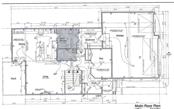
Main Floor Plan 1196 sf 9'1" Ceiling
